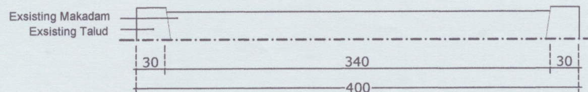
EXISTING JP4 Skala 1: 40
