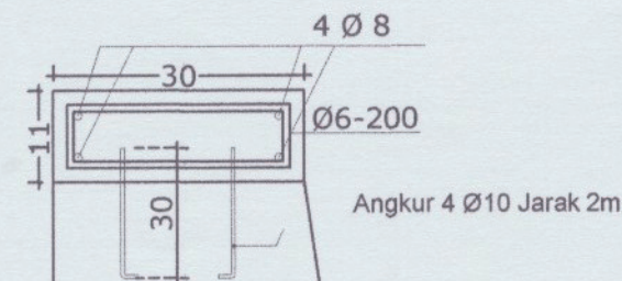
TYPICAL KANSTIN SLOOF 30x11 Skala 1: 20
