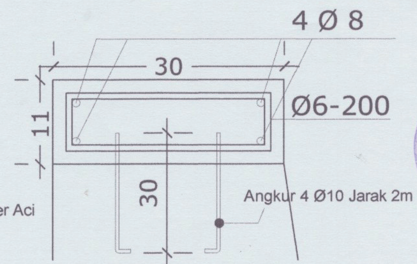
TYPICAL KANSTIN SLOOF 30x11 Skala 1:10
